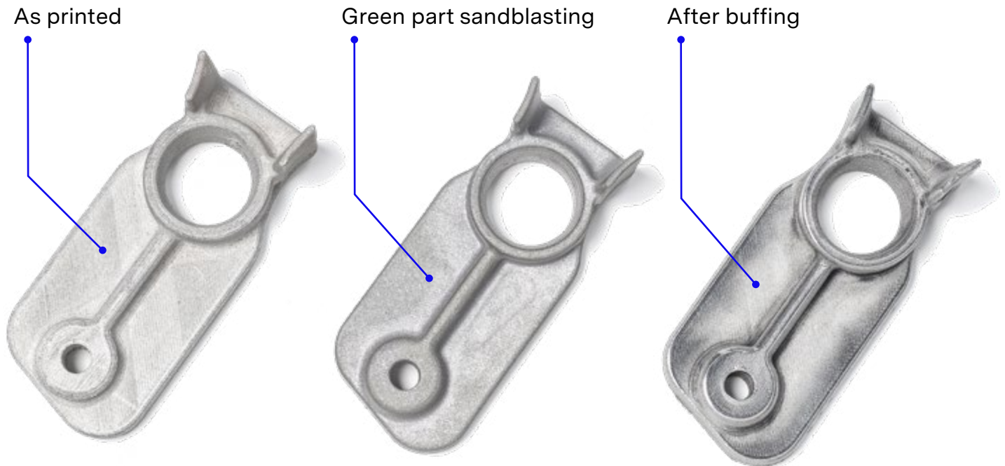
Figure 3: Results of different surface finishing for Liebherr Components' assembly tool
