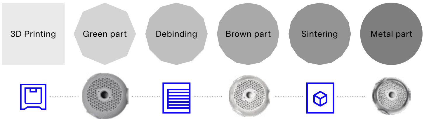
Figure 1: The Metal FFF process
