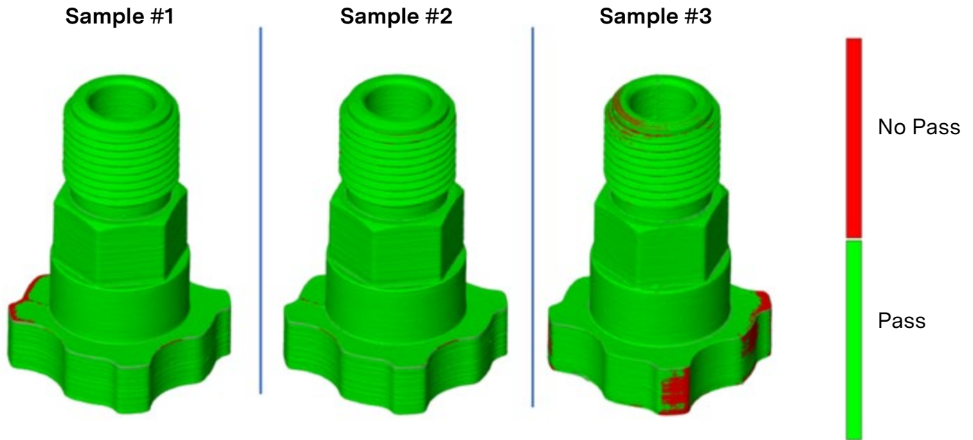
Figure 8: Color map generated through a pass/no pass filter with a threshold of \pm 0.3\text{mm} for the 3 adaptors printed and sintered
