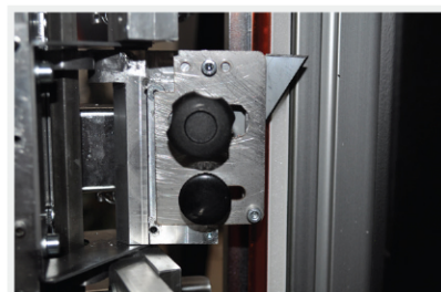
Fixed blade "2" Thickness from 1 to 10mm.
